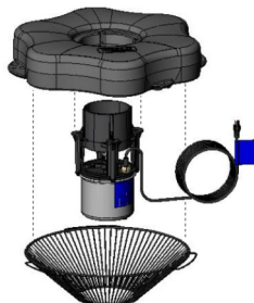
The motor unit attaches using stainless steel hardware. Single section, U.V. resistant, high density thermoplastic float. Bottom screen to protect the unit from debris.
